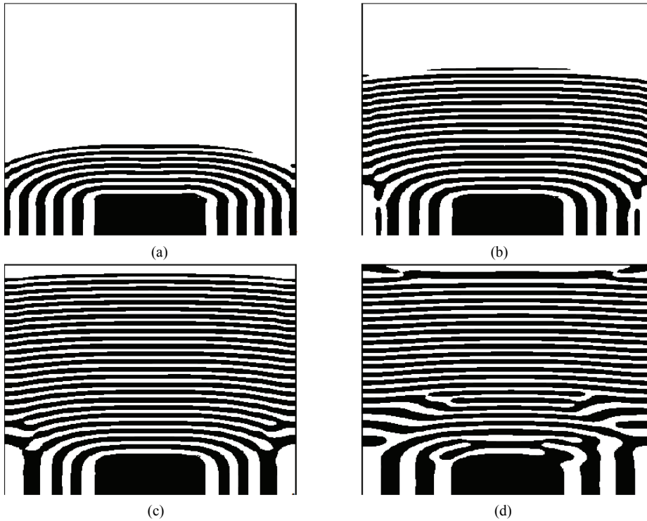
Figure 4. Time-development of crystallization process in the case of isotropic surface tension of crystal grains. The banding structure is transformed to the equiaxial structure: (a) t = 4 ; (b) t = 8 ; (c) t = 18 ; (d) t = 22 .
